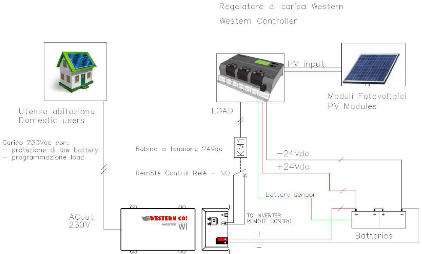
Pic. 4 WI400-24 Wiring scheme
